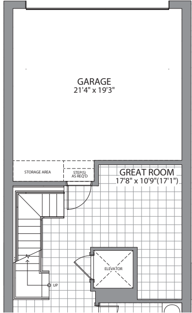
GROUND FLOOR W/ ELEVATOR OPTION
