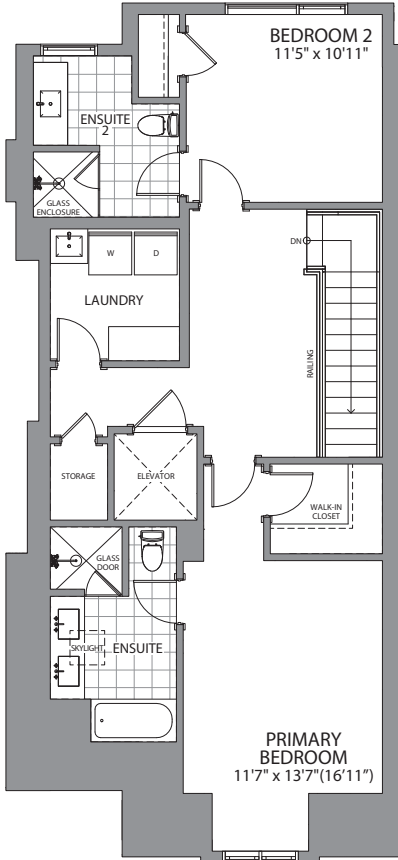
THIRD FLOOR W/ ELEVATOR OPTION
